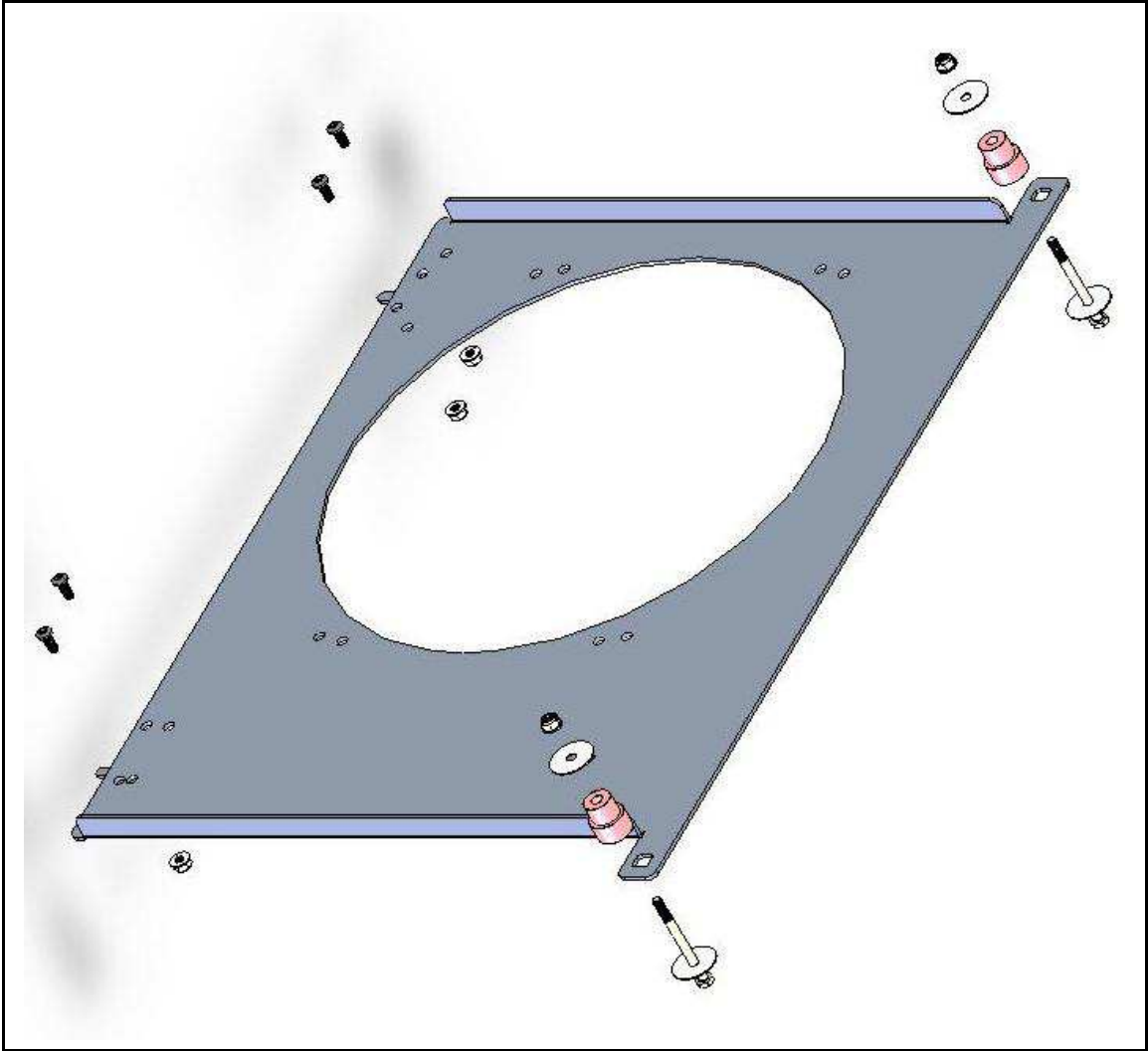
Figure 4: Fan mounting hardware
